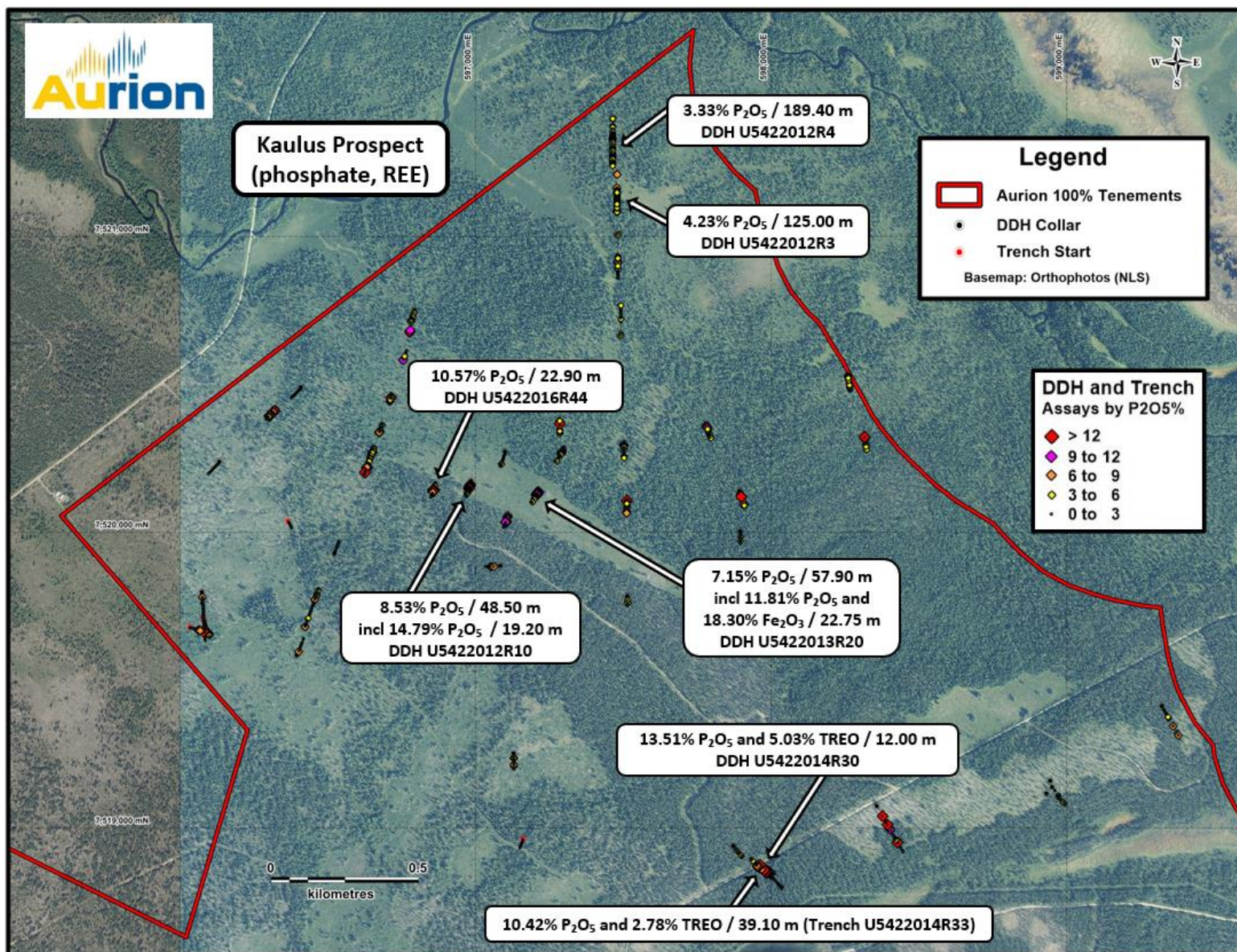
Figure 3: Kaulus phosphate-REE prospect. Location of historic drill holes and trenches with selected mineralized intervals.
