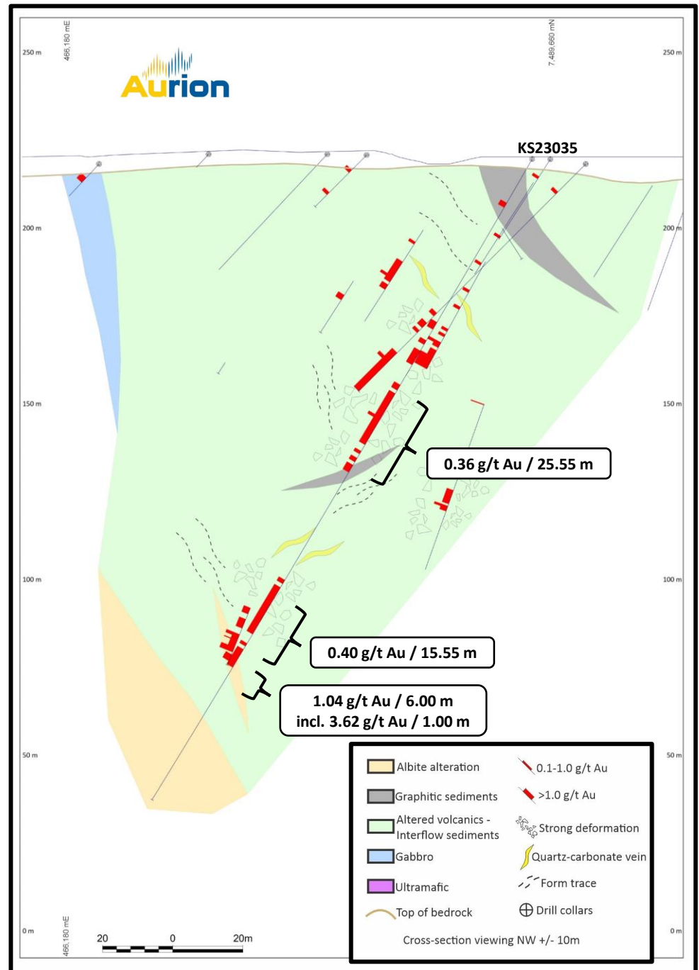
Figure 4: Cross section, hole KS22035.
