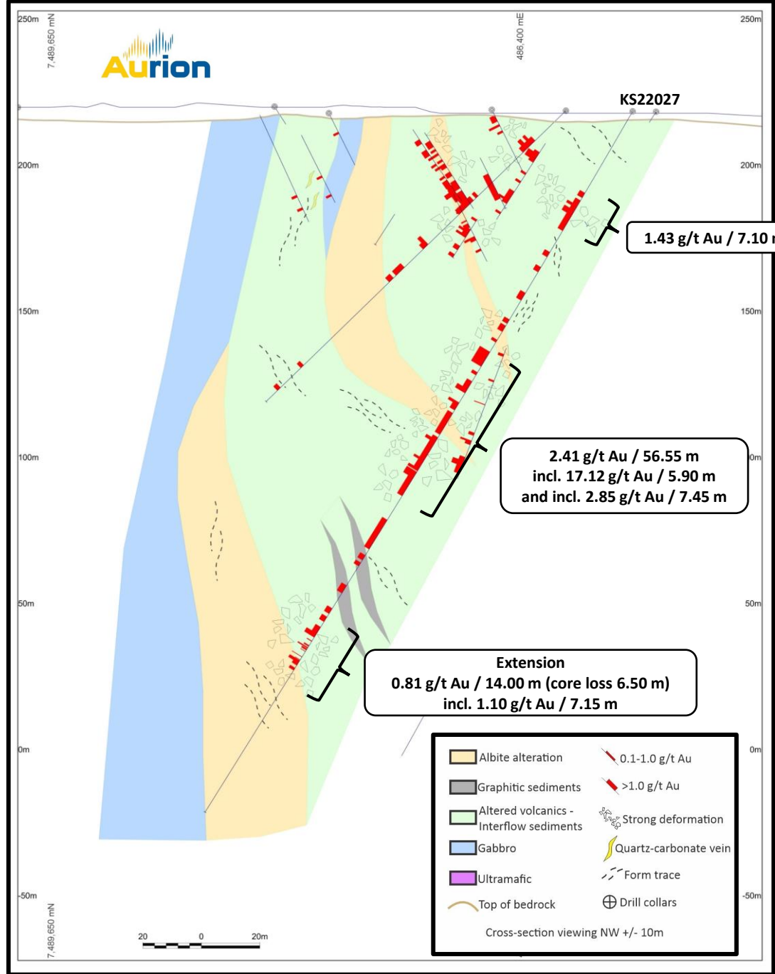
Figure 3: Cross section, hole KS22027.
