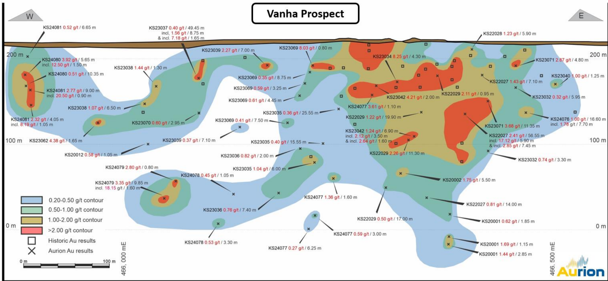
Figure 4: Schematic long section of the Vanha prospect, Kaaresselkä area, Risti property.
