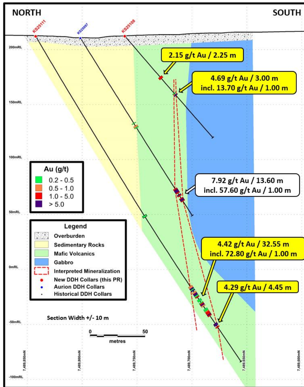
Figure 4: Schematic cross section (looking east) of the Vanha prospect, Kaaretselkä area, Risti property.
