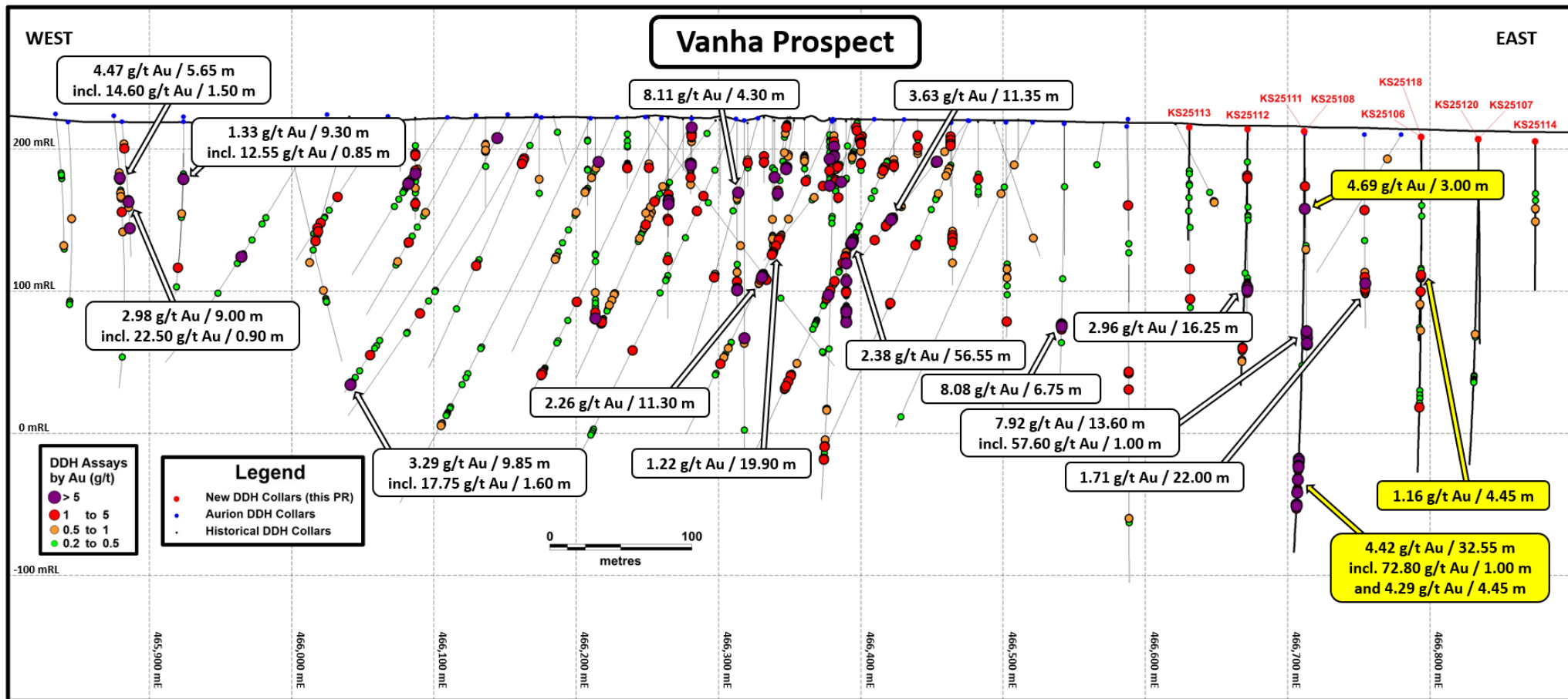
Figure 3: Schematic long section (looking north) of the Vanha prospect, Kaarelselkä area, Risti property.
