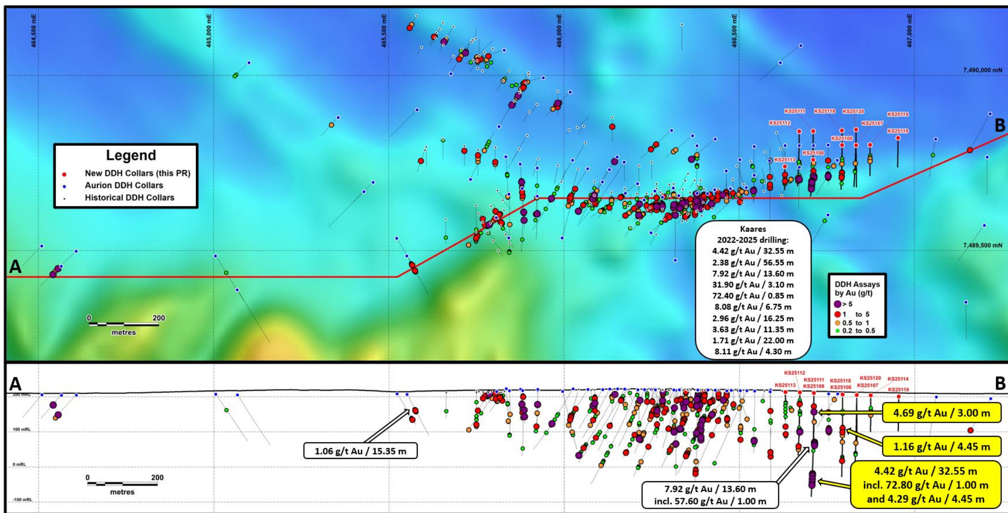
Figure 5: Schematic plan view and long section (looking north) of the Karesselkä area, Risti property.
