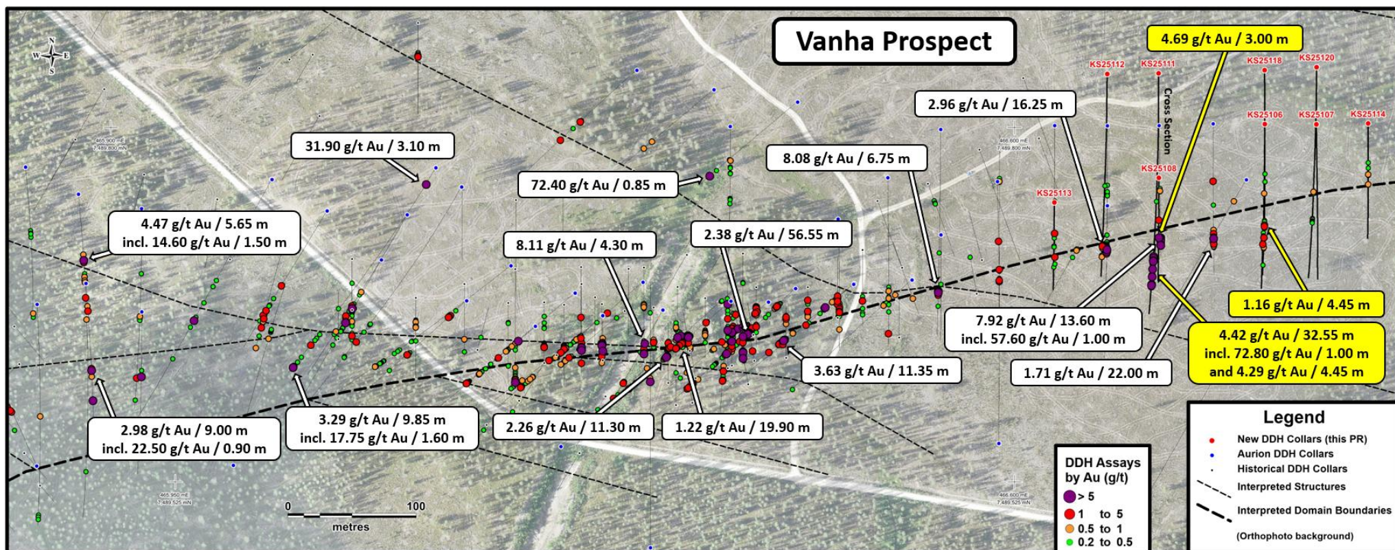
Figure 2: Drill holes at the Vanha prospect, Kaarelselkä area, Risti property.
