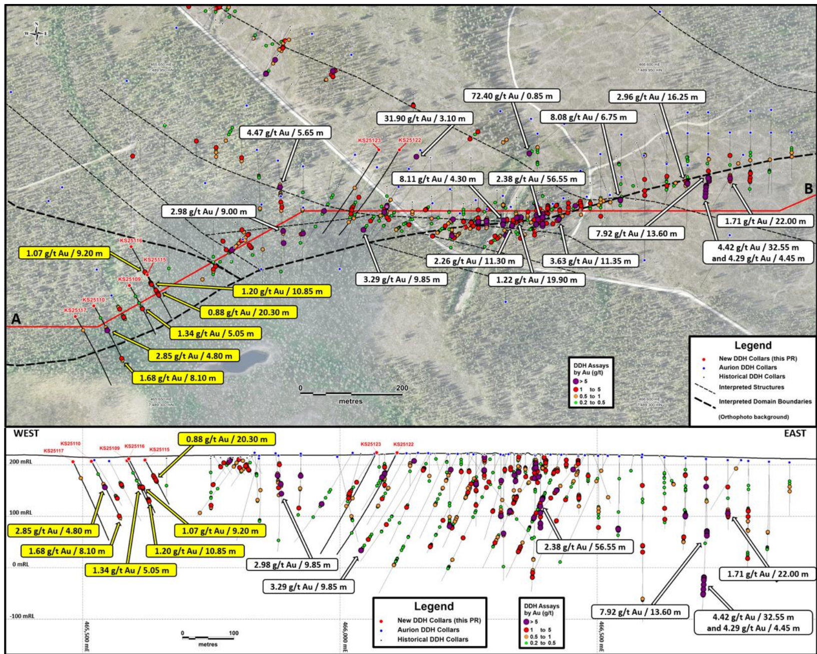
Figure 2: Drill holes at the Vanha prospect, Kaarelselkä area, Risti property.
