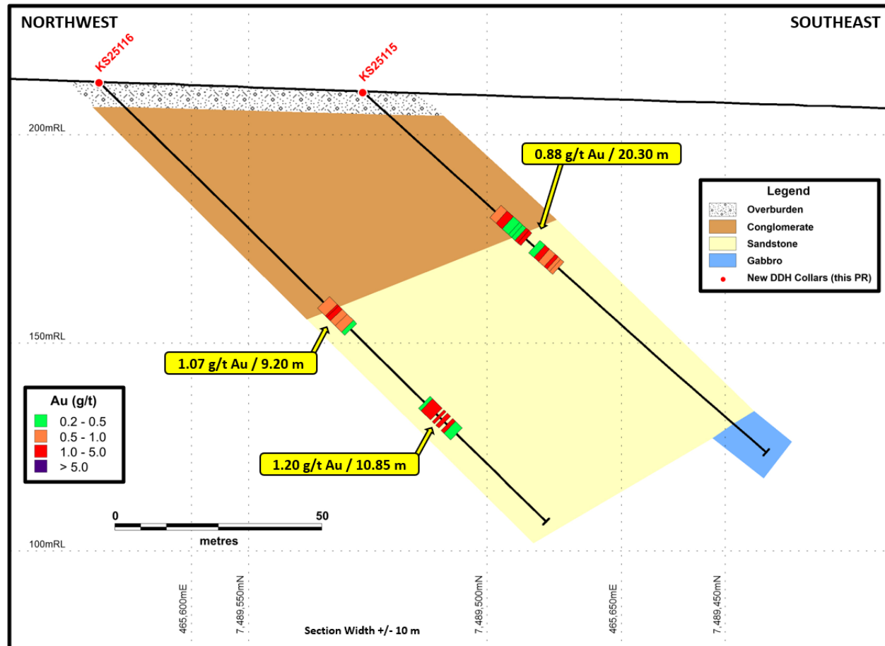
Figure 3: Schematic cross-section (looking northeast) at the western part of the Vanha prospect, Kaarelselkä area, Risti property.
