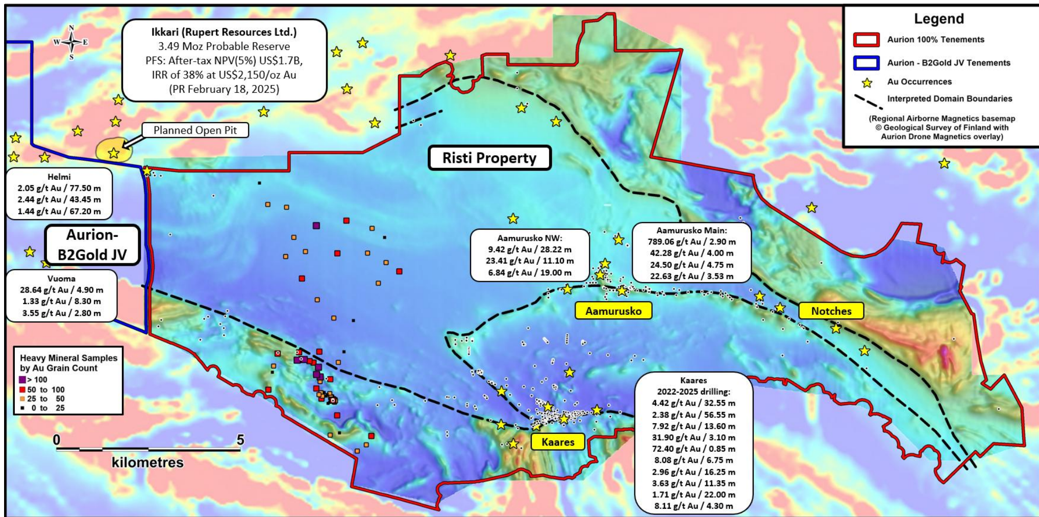
Figure 1: Map of the Risti property (Aurion 100%) with drill hole collars, heavy mineral samples and gold occurrences.
