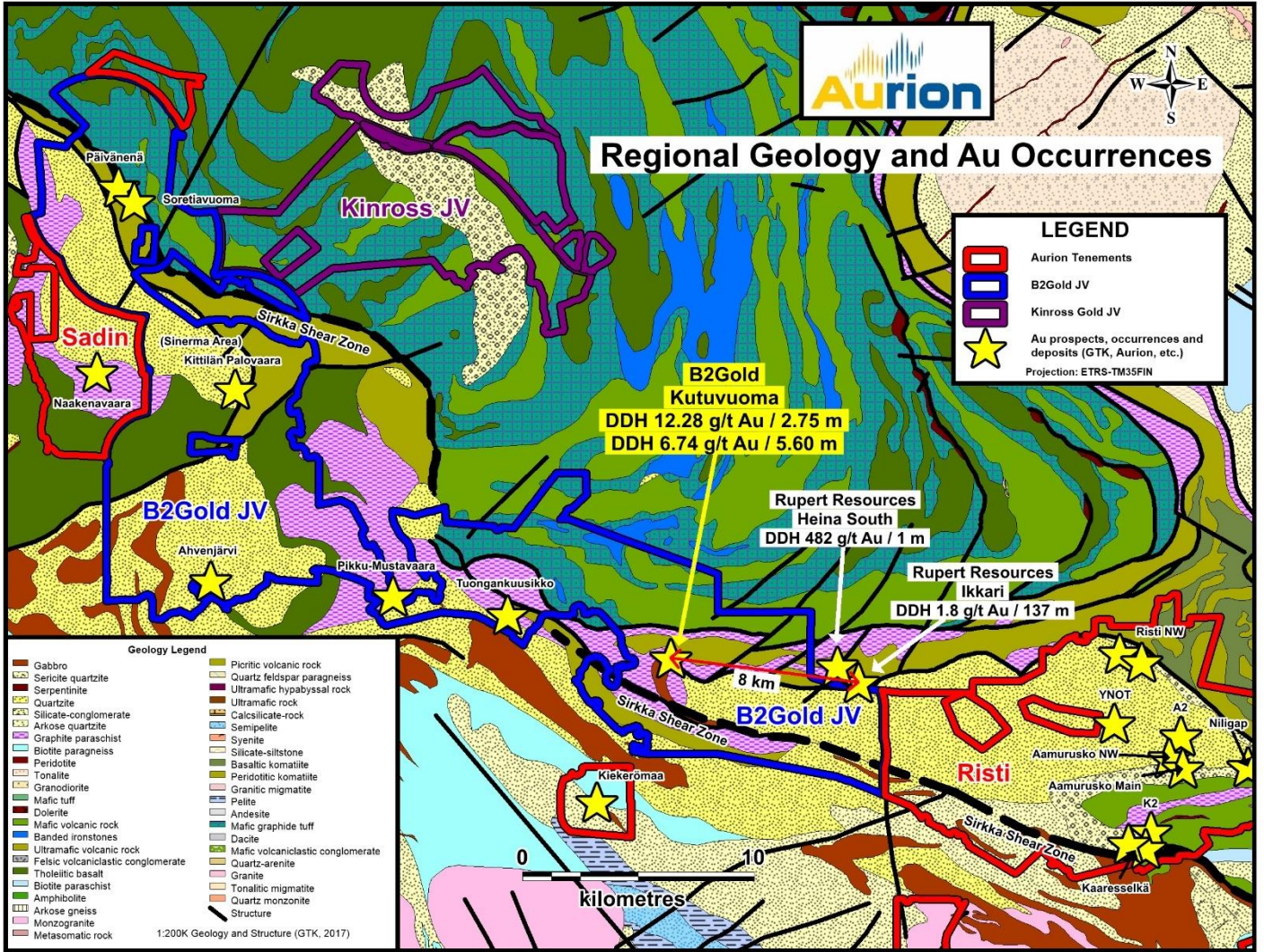
Figure 1: Regional Geology
