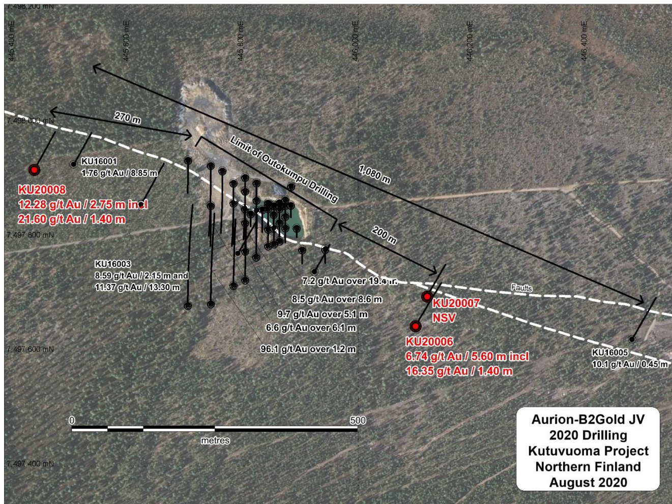
Figure 2: Drill Plan Map
