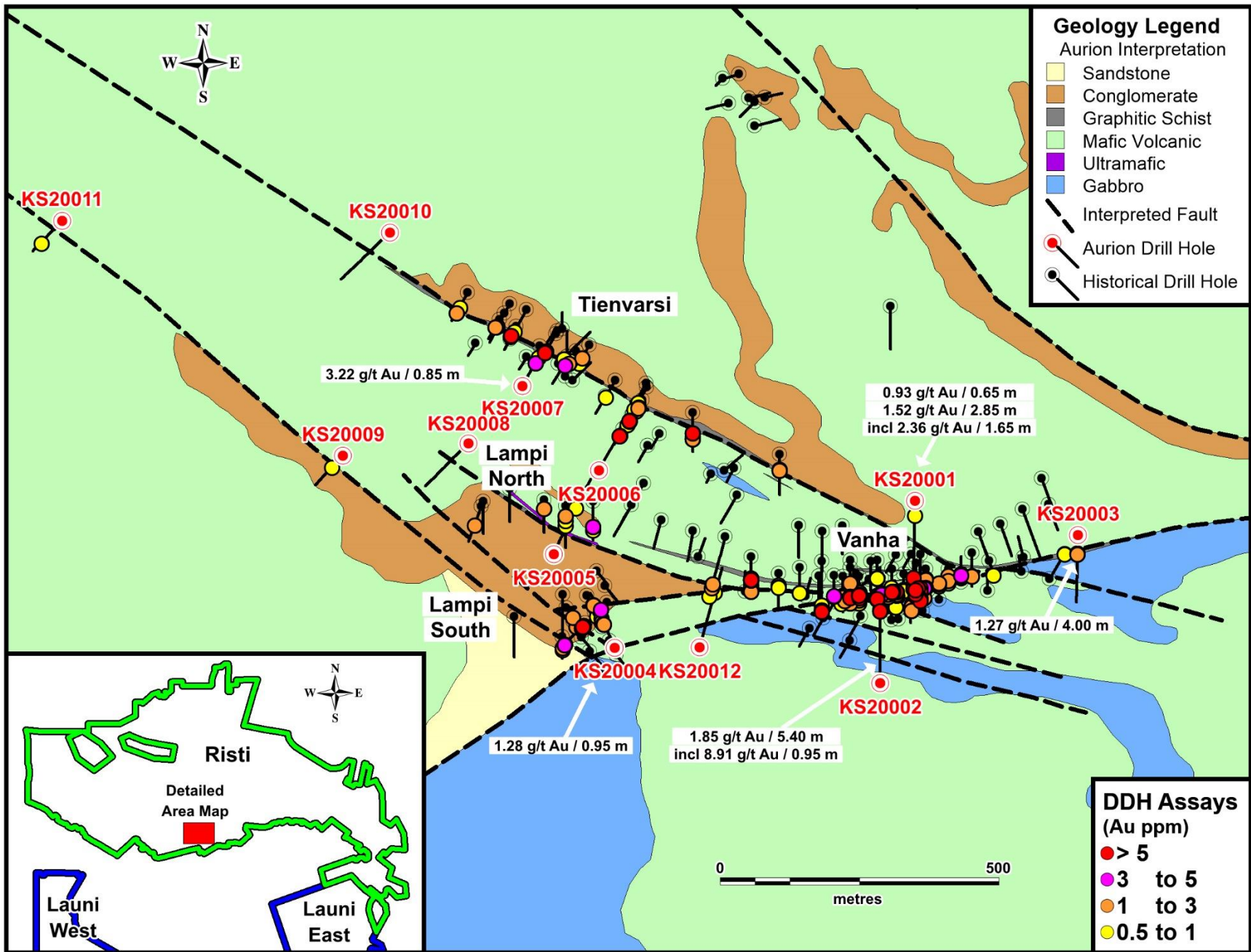
Figure 2: Karesselkä Plan View
