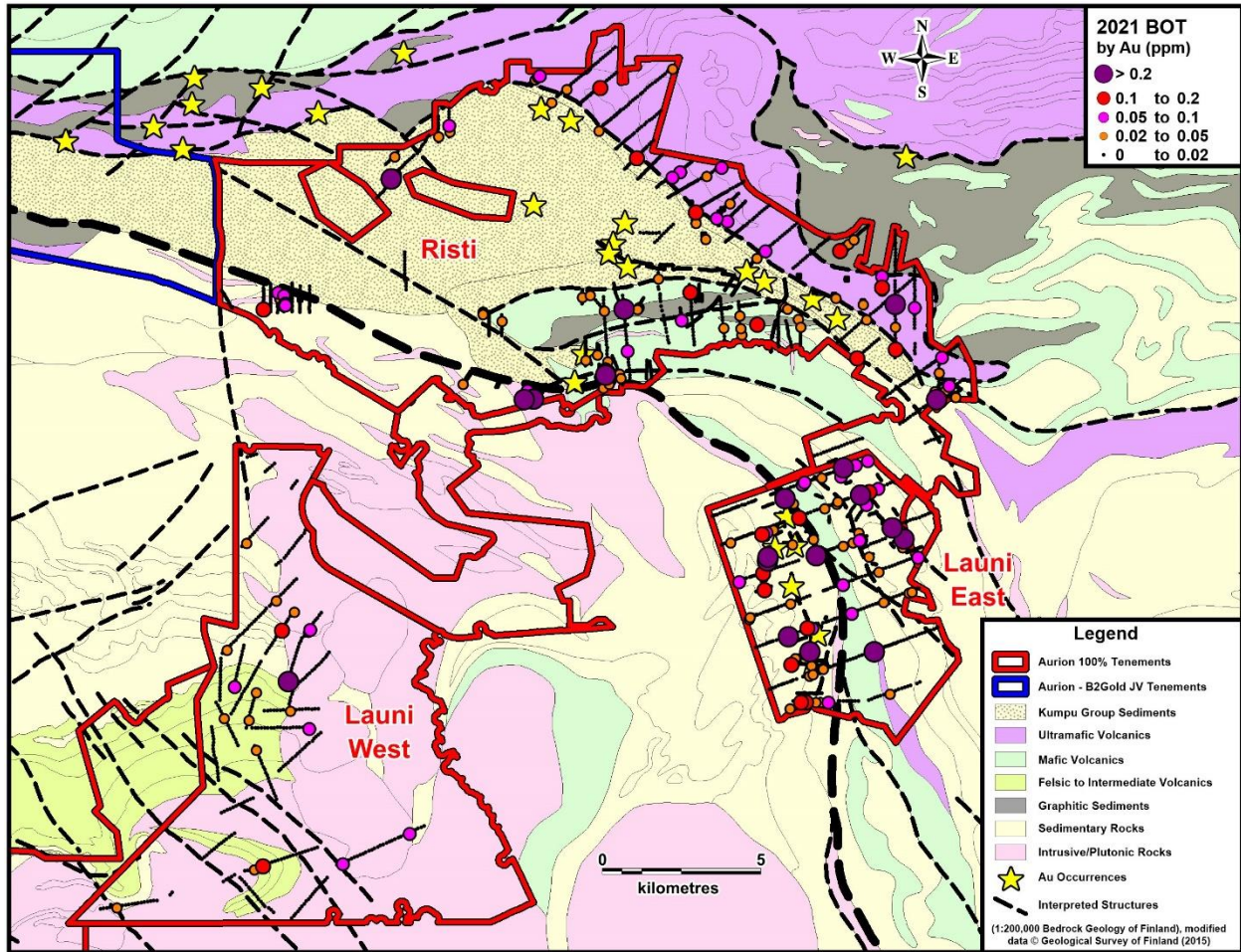
Figure 2: Geology map and base of till samples at Risti and Launi properties.
