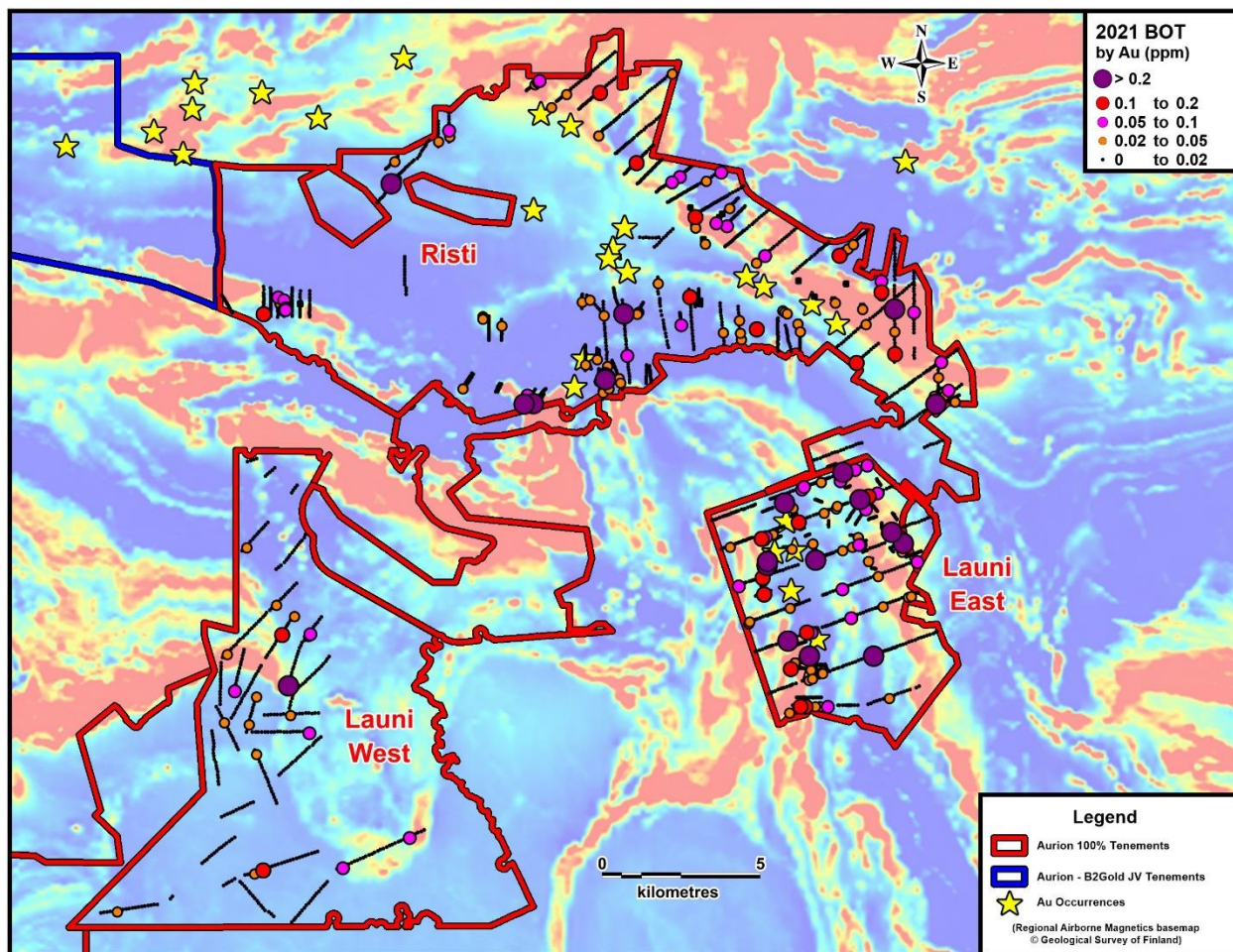
Figure 3: Airborne magnetic geophysical map and base of till samples at Risti and Launi properties.
