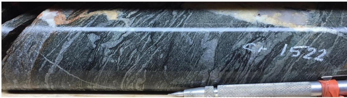
Qtz-Mt-Py vein (left) in chlorite-sericite altered ultramafic tuff (16.2m).
